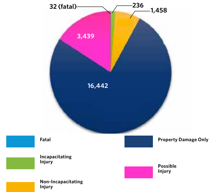
FIGURE 4.3 CRASH SEVERITY, 2013-2017
